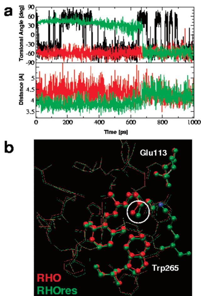
FIGURE 3: Study of the absolute conformation of the chromophore. (a) Top panel: \varphi_{H-C10-C13-C20} of the chromophore in water (SOLcis, black line), in RHO (red line), and in RHOres (green line). Bottom panel: Distance between C20 and the closest carbon atom of Trp265. (b) Comparison of the average structures of simulations RHO (red) and RHOres (green), where the torsional angle \varphi_{H-C10-C13-C20} is restrained to a positive value. The two structures differ only in the position of the C20 methyl group that comes into contact with Trp265 in RHOres.
